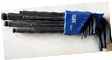
Hex Key Set, ball, Metric, 9PC. Sizes: 1.5 to 10
